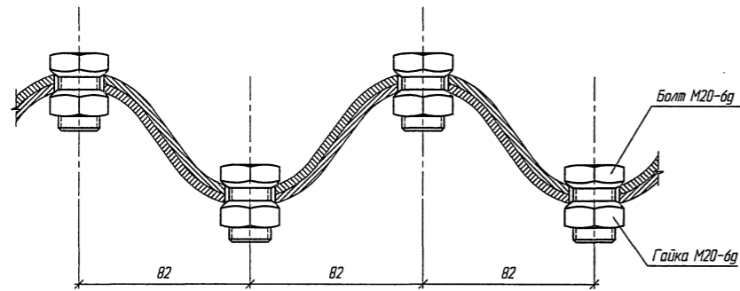
2-2
