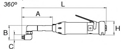
LBV16, -25 360°
