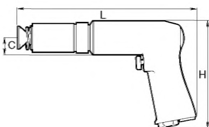
RRH
