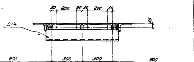
2-2
