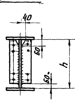
По 2-2
