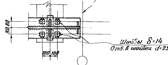
По 4-4
