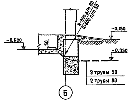
2-2; 3-3
